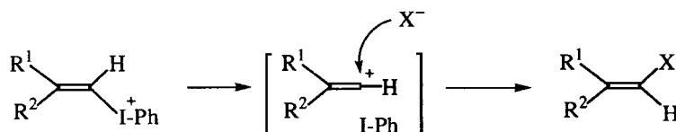
Scheme 2. Ion-pair mechanism.
